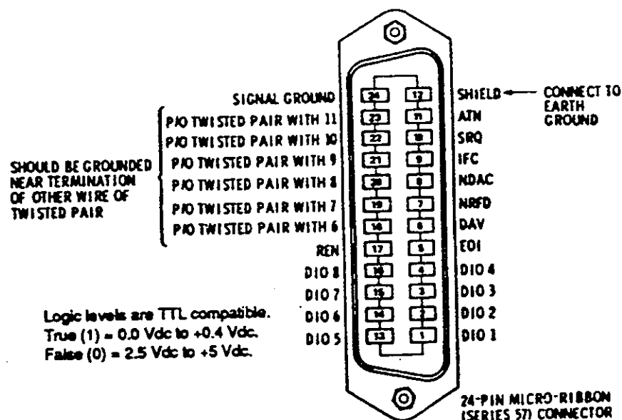
Figure 3-8. GPIB Wiring Connector Pin Out
