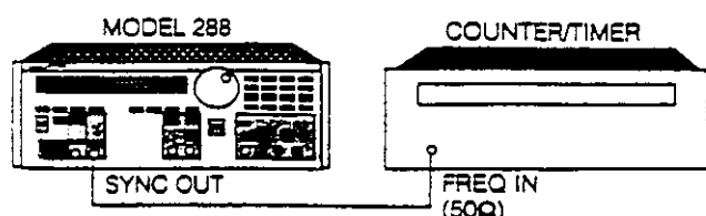
Figure 2-2. Frequency Measurement Setup
