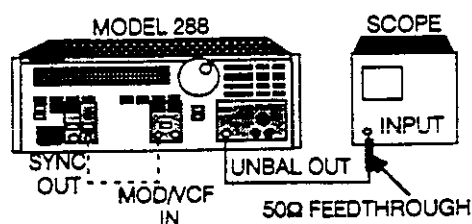
Figure 5-5. Adjust AM Setup
