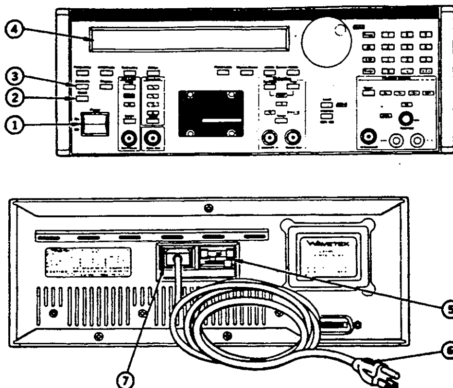
Figure 2-1. Equipment Setup
