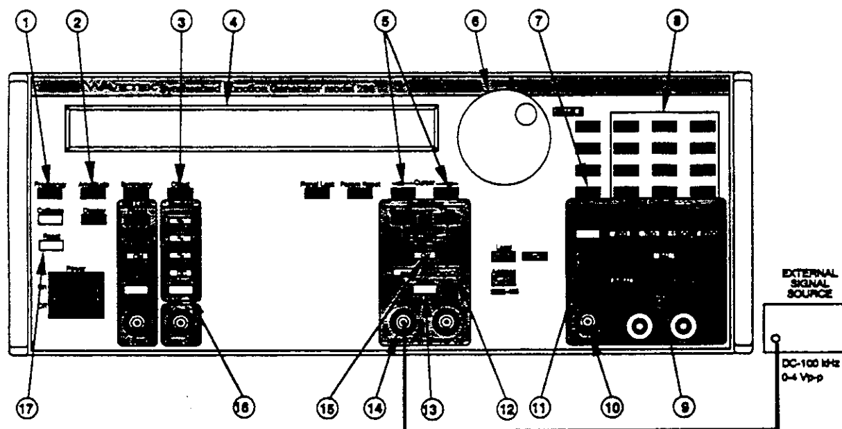
Figure 3-6. Frequency Modulation Operation Control Setup
