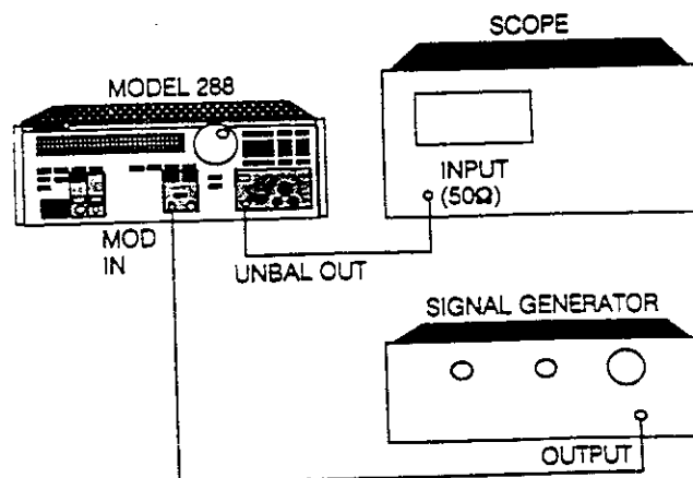
Figure 2-6 AM Verification
