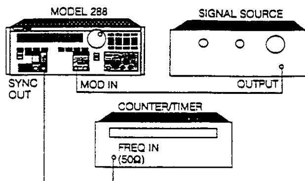
Figure 2-3. VC/FM Setup
