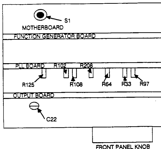
Figure 5-1. Calibration Location
