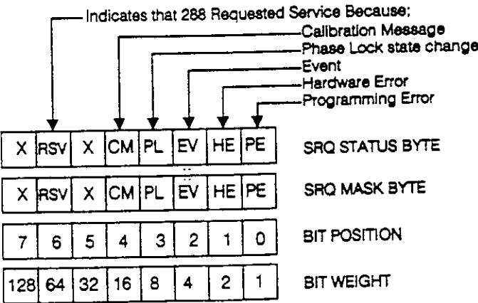
Figure 3-11 Model 288 Status Byte and SRQ Mask
