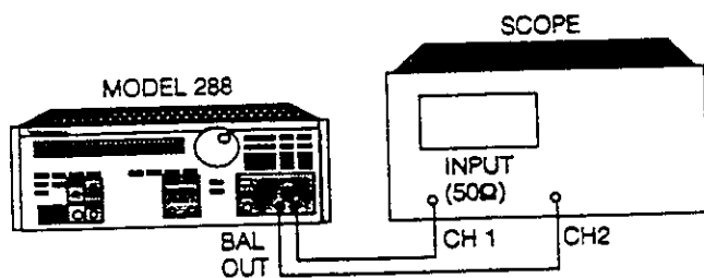
Figure 2-5. Balanced Output Verification
