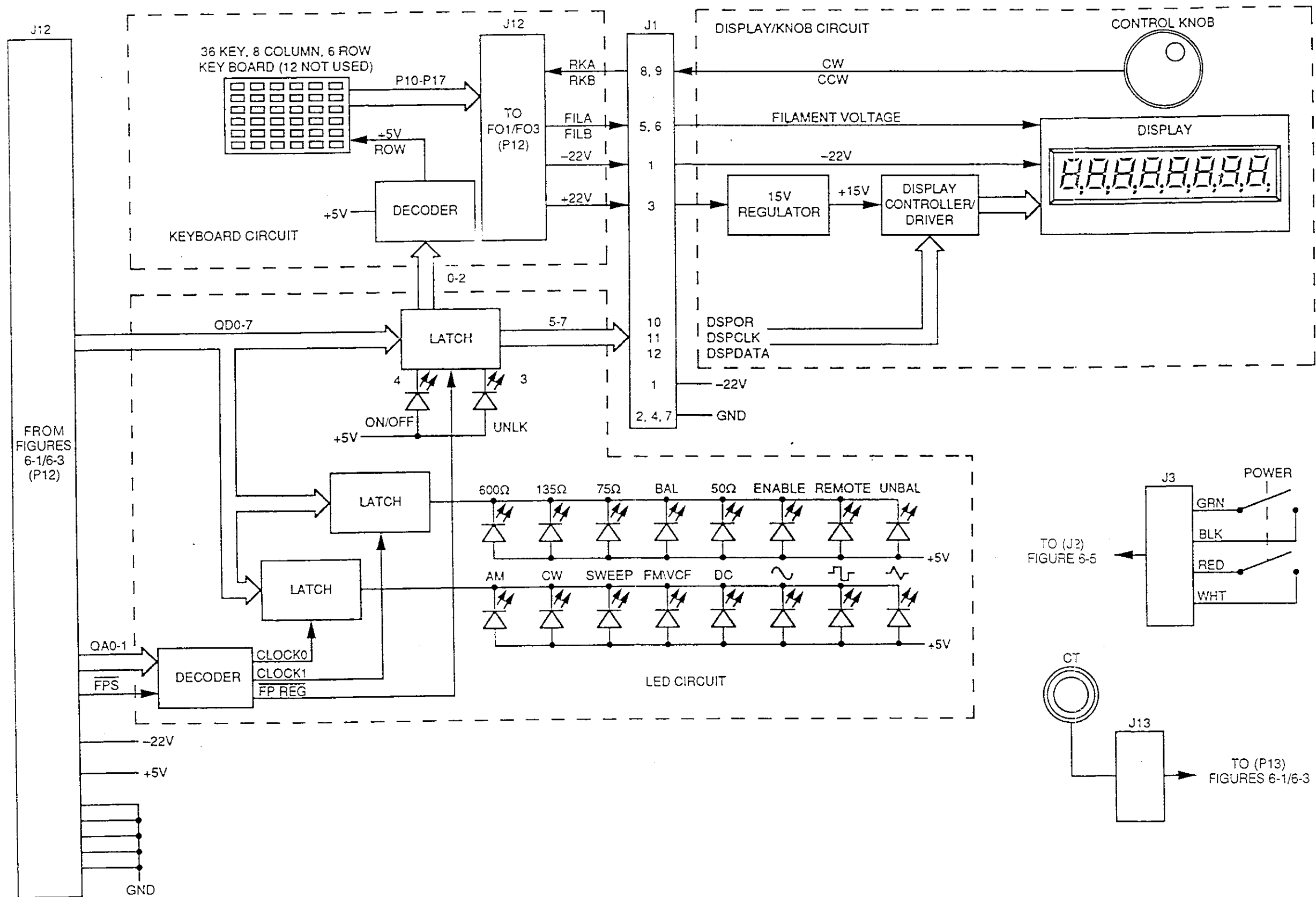
Figure 6-2. Front Panel (Sheet 2 of 2).
