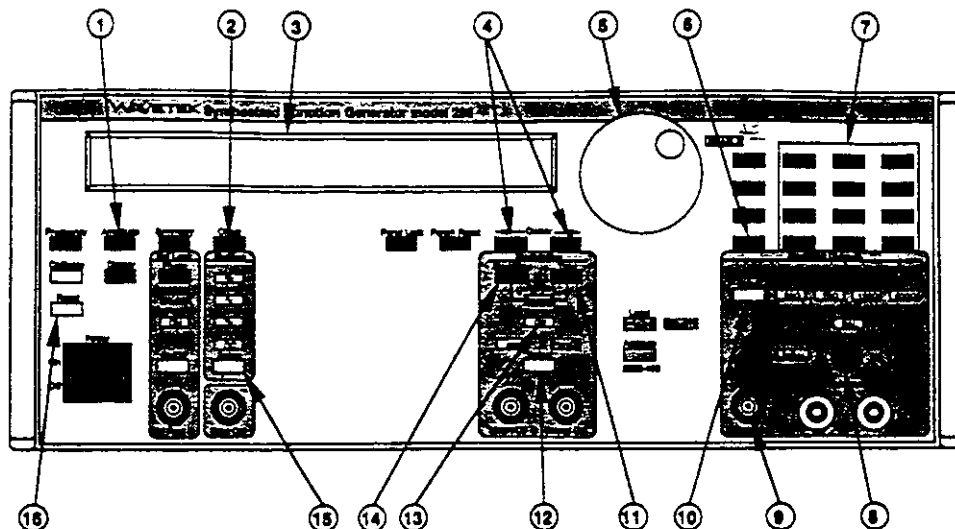
Figure 3-4. Sweep Modulation Operation Control Setup
